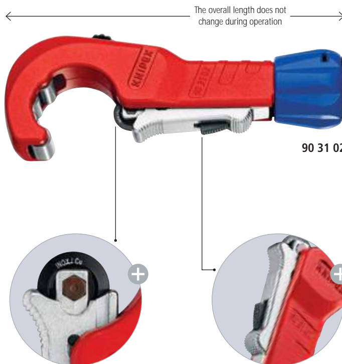
The needle-bearing and spring-loaded cutting wheel made of high-quality ball bearing steel is easily exchangeable
