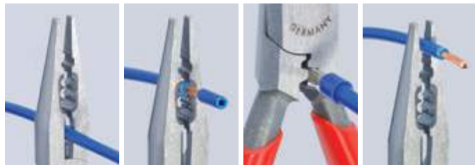
Cutting Edges Stripping Crimping 0.5 to 2.5 mm 2 Gripping
